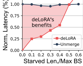
Figure 20. Latency gain of mixture mode.
