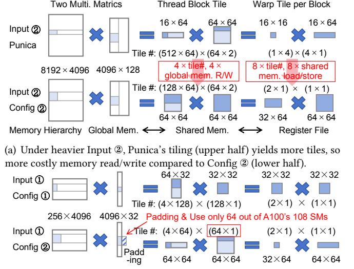
(a) Under heavier Input ②, Punica’s tiling (upper half) yields more tiles, so more costly memory read/write compared to Config ② (lower half). (b) But under lighter Input ①, Config ② (lower half) cannot deliver good performance because it underutilizes SM since fewer block number.
